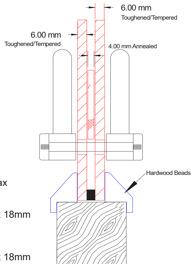
Non Fire Rate Bead Details Cross Section Vistamatic Max Panel
